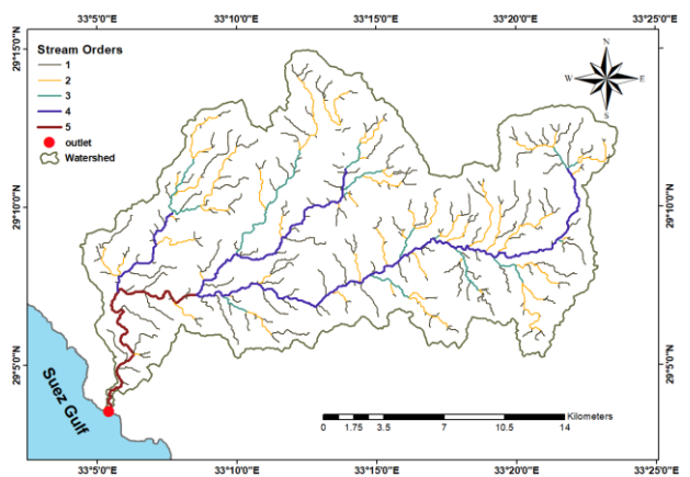
Figure 14 Stream orders of wadi Tayyibah.
