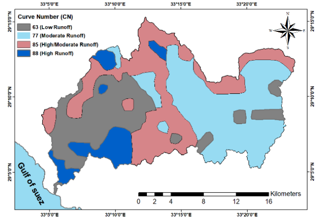
Figure 10: Values of CNs of Wadi Tayyibah.
