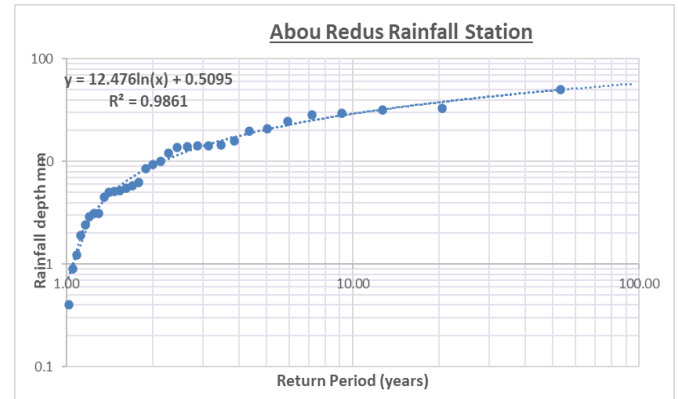
Figure 9: Best fit distribution graph for Abou Redus Station.
