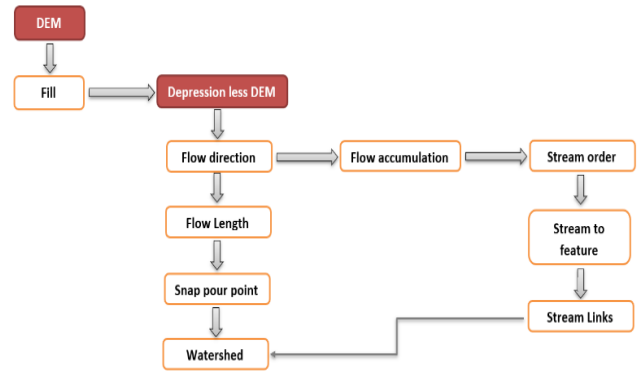
Figure11 steps of Watershed delineation.
